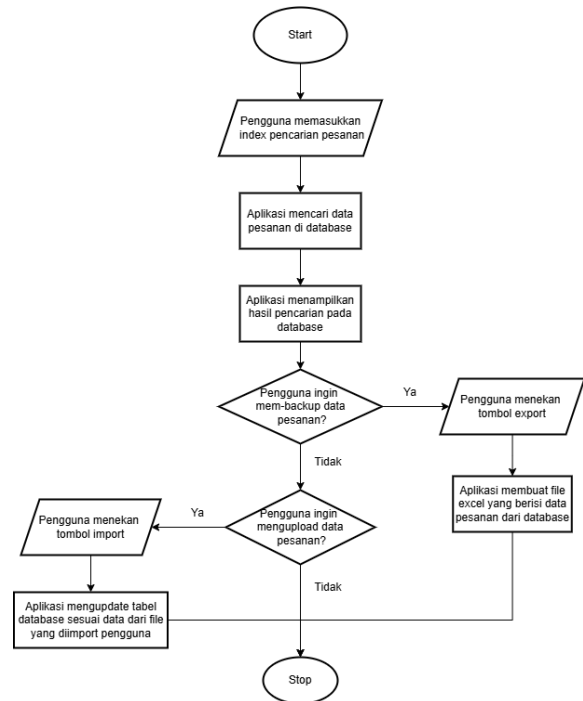
Gambar 5. Flowchart fitur “histori pesanan”
