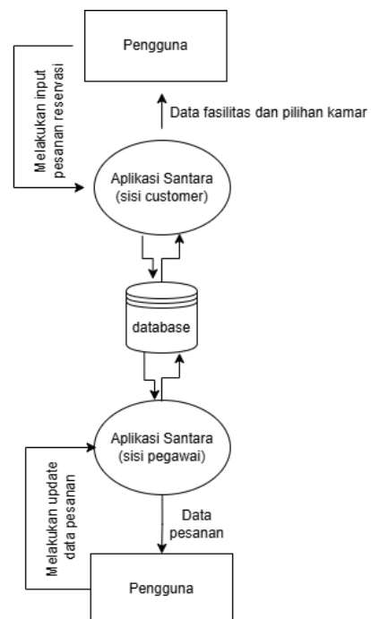
Gambar 7. Diagram Aliran Data
